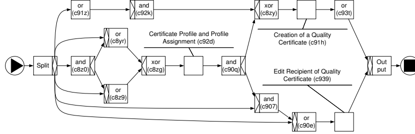
Fig. 3. YAWL model obtained by applying the mapping shown in Fig. 2 to the example of the top four connectors in Fig. 1. Moreover, from the initial OR-split task “Split” we only consider the arcs connected to these four dummy tasks.
