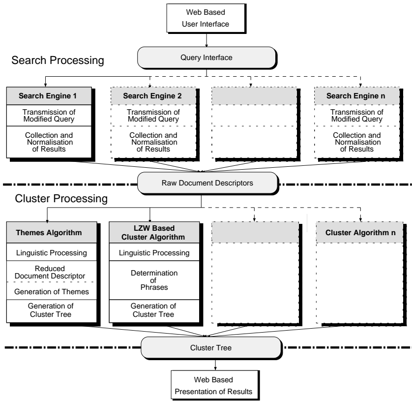
Figure 1: Architecture of MSEEC
