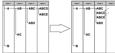
Figure 5: Limiting the Depth of the Cluster Tree.
