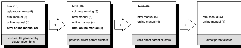
Figure 4: Example of finding a direct parent cluster of html online manual.
