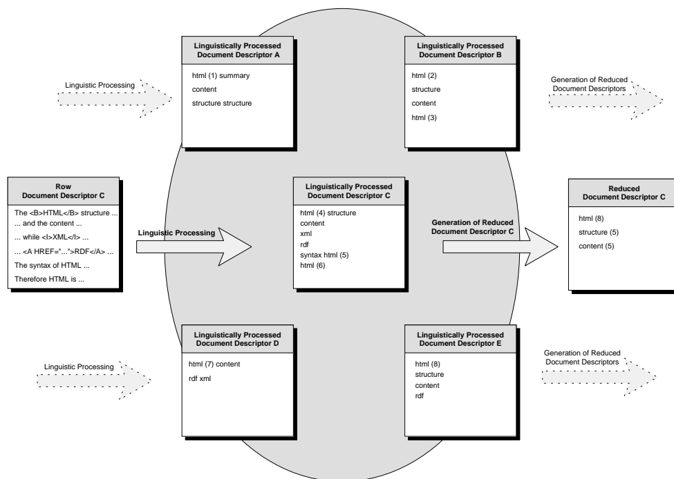
Figure 3: Example for the Generation of a Reduced Document Descriptor
