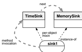
Figure 9: Time Sink as Mixin
