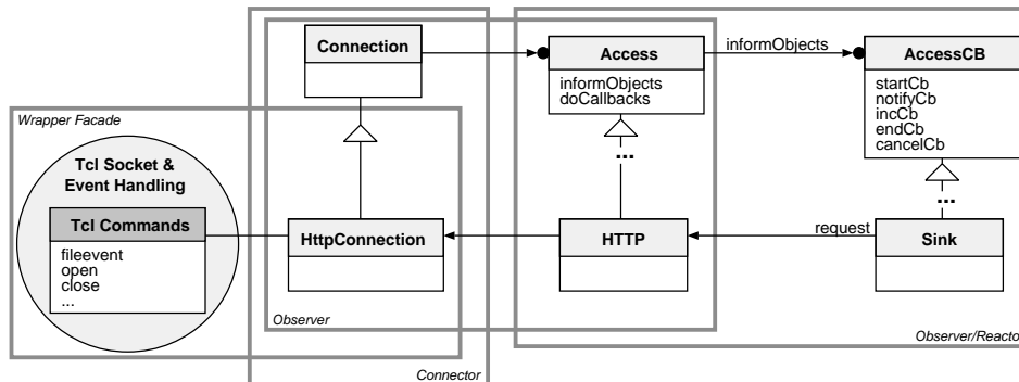
Figure 4: Callback Interface and Reactive Event Handling
