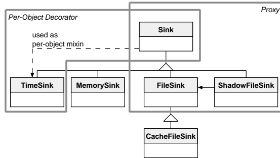
Figure 7: Sink Classes
